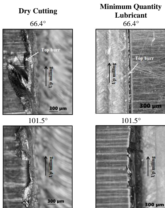
Figure 9. Burr formation under different swept angles and cutting conditions
