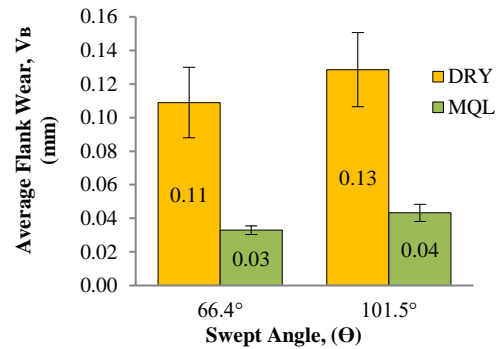
Figure 3. Average flank wear under different swept angles and cutting conditions
