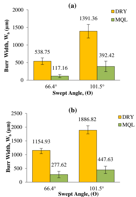
Figure 10. Average burr width under different cutting condition after (a) 1 st slot; and (b) 10 th slot
