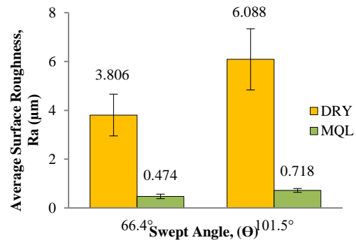
Figure 7. Average comparisons for surface roughness, R_a .
