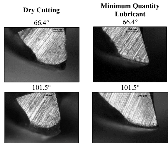
Figure 4. Tool wear growth for both different swept angles and cutting conditions
