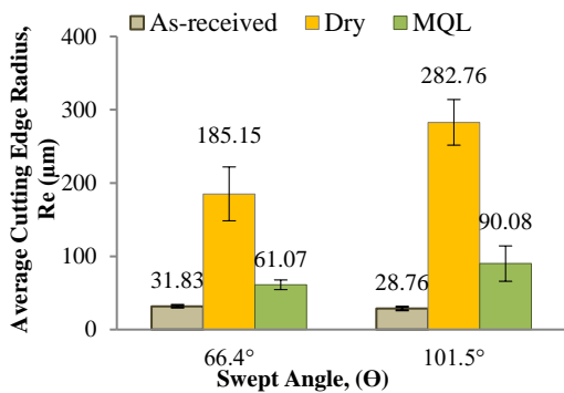
Figure 6. Changes of cutting-edge radius for both swept angles and cutting conditions
