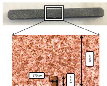
Figure 2. BGC/ ZrO 2 composite specimen after created Notched using SENB method
