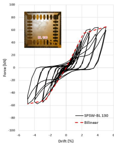
Figure 14. The hysteresis curve of BL 130 specimen and the ideal bilinear curve
