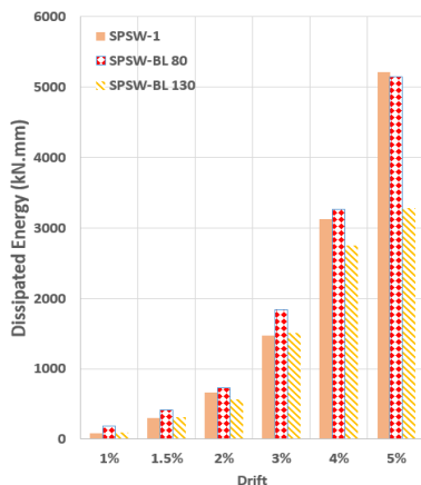
Figure 15. Comparison of energy dissipated by laboratory specimens at each drift
