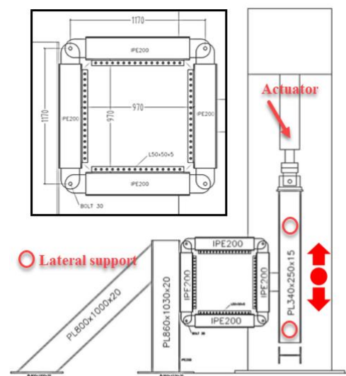
Figure 3. Specimen setup and loading system
