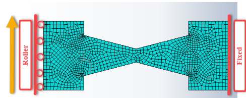
Figure 16. The butterfly-shaped link modeled in Abaqus
