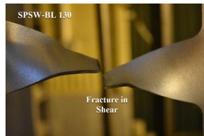
Figure 11. Link fracture in BL 130 specimen
