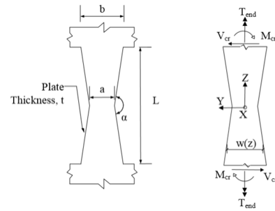
Figure 1. Butterfly fuse, geometry and internal forces [22]
