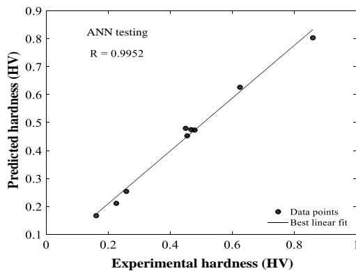
Figure 6(a). Regression analysis of predicted and experimental hardness for testing data
