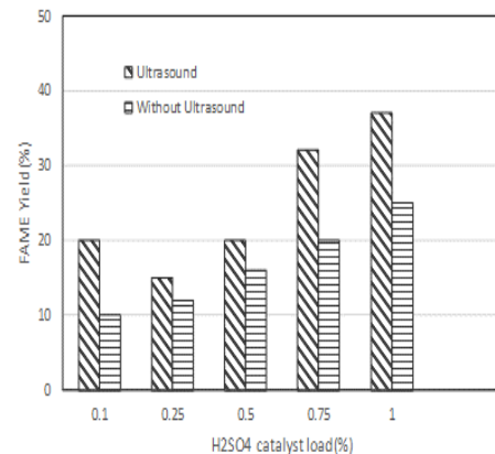
Figure 3. Effect of catalyst concentration on yield of FAME for experiment without and with ultrasound
