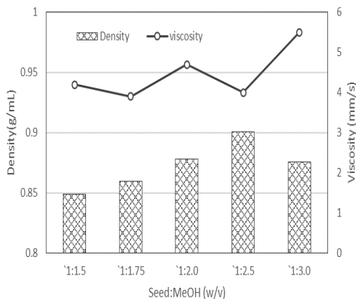
Figure 4. Effect of raw material ratio to methanol on density and viscosity of biodiesel
