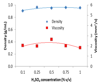
Figure 2. Effect of catalyst concentration (v/v%) of H 2 SO 4 on density and kinematic viscosity of biodiesel
