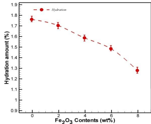
Figure 8. Effect of nano Fe_2O_3 addition on improvement of hydration resistance of samples.
