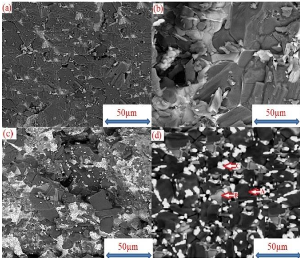
Figure 7. SEM images of fractured surfaces of the samples with a) without, b) 2%, c) 6% and d) 8wt. % nano ZrO_2
