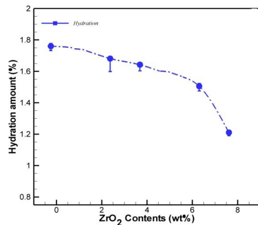
Figure 9. Effect of nano ZrO_2 addition on improvement of hydration resistance of samples.
