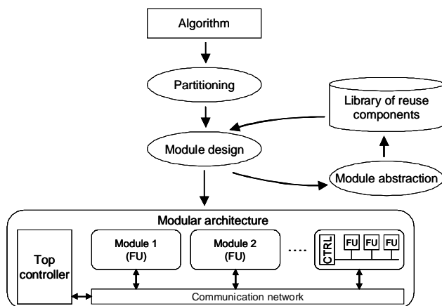
Figure 2. Modular design flow
