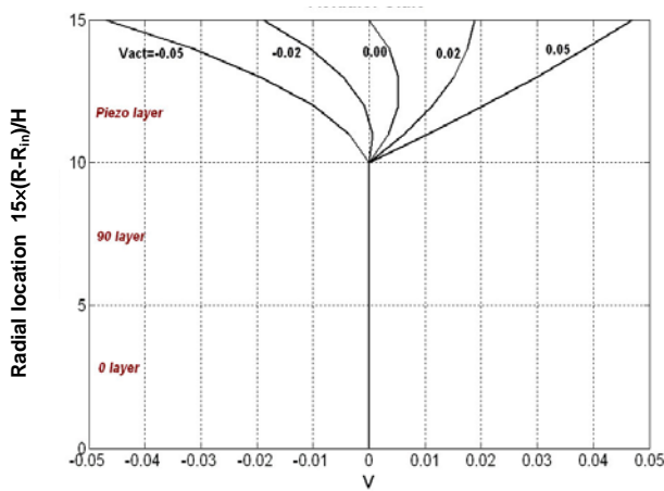
Figure 5. Actuator voltage distribution at the middle (i.e., at \theta = 22.5^\circ ) of 45^\circ - panel subjected to outer pressure.
