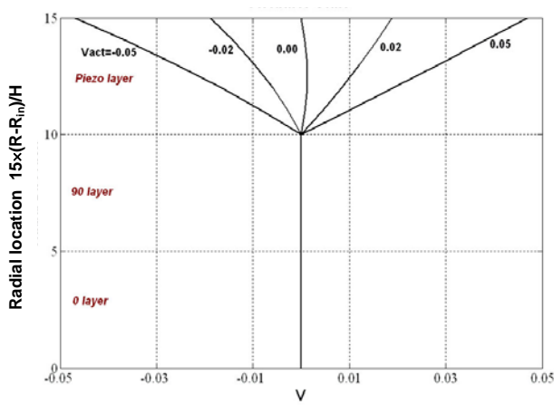
Figure 6. Actuator Voltage Distribution at the Middle (i.e., at \theta = 11.25^\circ ) of 22.5^\circ - Panel Subjected to Outer Pressure.
