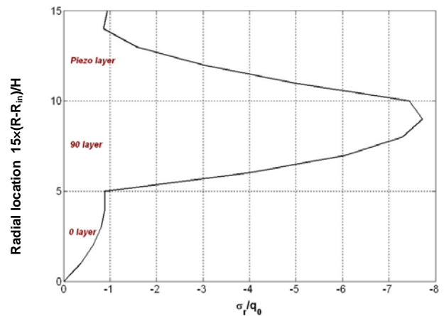
Figure 7. Through-thickness distribution of radial stress at the middle point (i.e., at \theta = 22.5^\circ ) of 45^\circ - Panel subjected to outer pressure.
