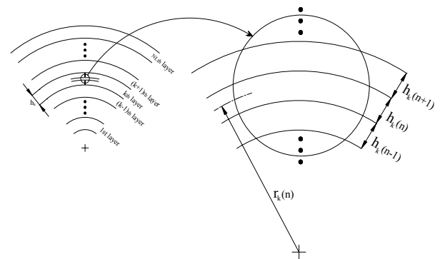
Figure 2. k^{\text{th}} layer is divided into N thin sublayers with thickness h_k(n), n = 1, \dots, N .
