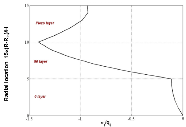
Figure 8. Through-thickness distribution of radial stress at the middle point (i.e., at \theta = 11.25^\circ ) of 22.5^\circ - panel subjected to outer pressure.
