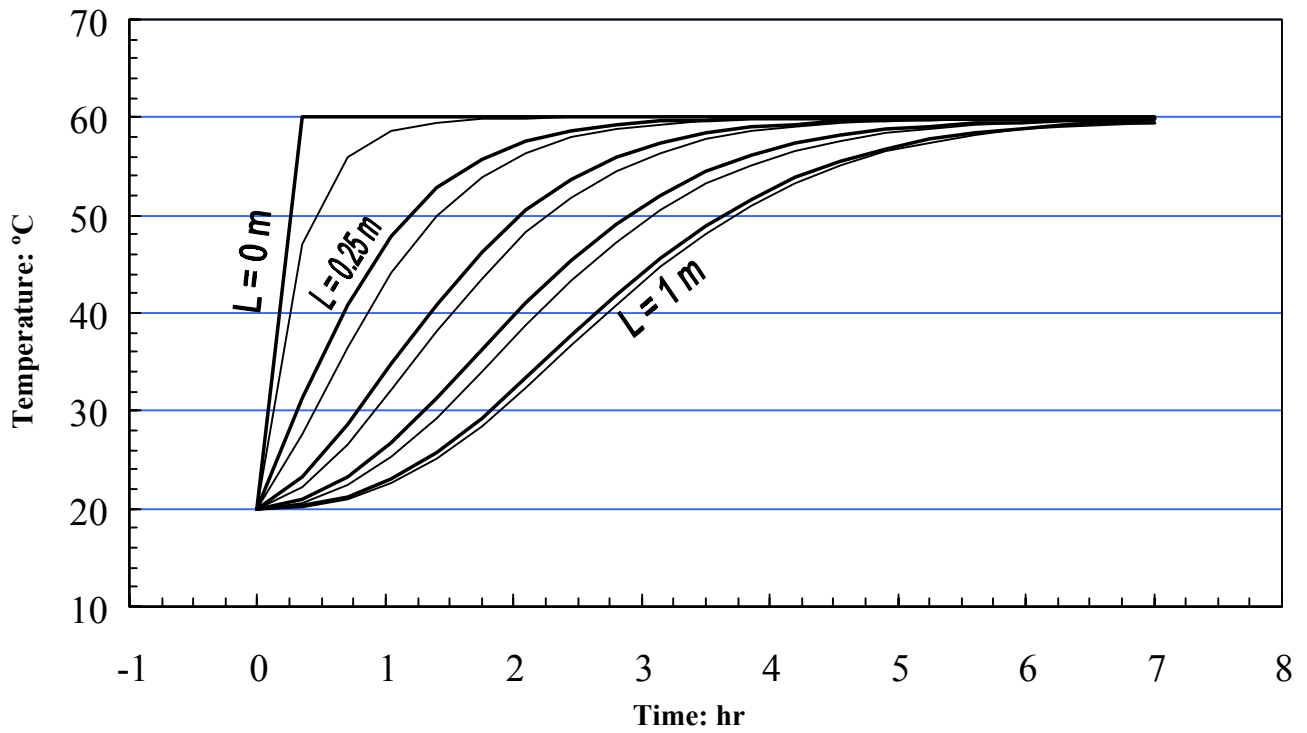
Figure 9. Comparison of air and rock temperatures variation in different Layers of rock bed.
