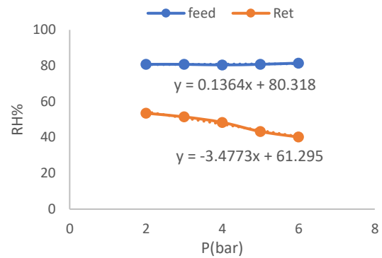
Figure 8. Diagram of changes in relative humidity of residue versus relative humidity of feed in the 1SiO_2 membrane
