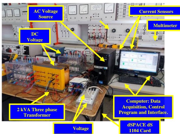
Figure 2. Measurement setup
