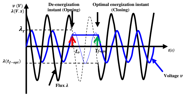
Figure 7. Voltage-flux relationship for optimal switching on
