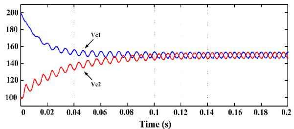
Figure 12. Dynamic balancing process of capacitors with initial voltage V_{C1} = 200\text{ V} and V_{C2} = 100\text{ V}
